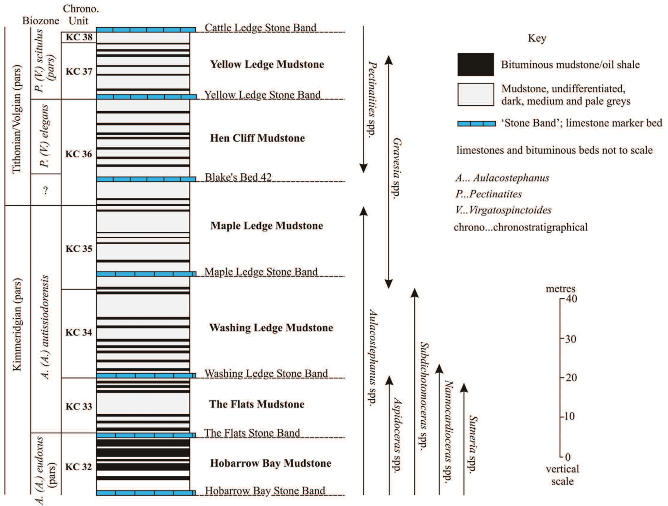
Figure 3. Simplified vertical section for the Kimmeridge Clay succession exposed in the cliff and foreshore sections between Hobarrow Bay and Cuddle showing the principal lithologies and ammonite ranges (after Cope, 1967, Cox and Gallois, 1981 and Van der Vyver MS, 1986), and the revised nomenclature (in bold) for the mudstones (Gallois, in press).
