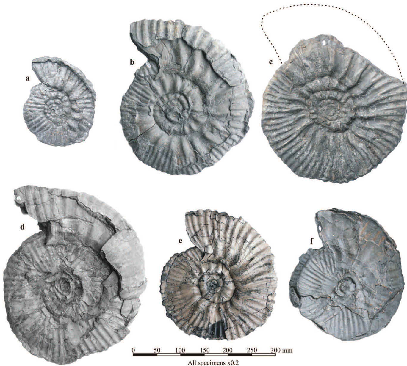
Figure 8. Examples of Gravesia from the elegans and scitulus zones in the Kimmeridge area. (a) Microconch or juvenile of Gravesia cf. gigas , K1324, Bed HC11, elegans Zone, foreshore below Hen Cliff. (b) G. cf. gigas (M), K508, Bed HC8, elegans Zone, foreshore below Hen Cliff; nodes weaker than those of G. gigas and more pronounced than the bullae of G. gravesiana . (c) G. cf. gravesiana (M), K1122, Bed HC15, elegans Zone, foreshore below Hen Cliff. (d) Gravesia sp.(M), K1332, Bed HC17, foreshore below Hen Cliff; fine ribbing and absence of bullae or nodes on the phragmocone distinguishes this example from the type specimens of G. gigas and G. gravesiana . (e) G. cf. gravesiana (M), K1647 Bed HC17, foreshore in Brandy Bay, bullae and ribbing similar to G. gravesiana , but shell details better preserved than in the type material. (f) Gravesia sp. (M) K1180, Bed Y10, scitulus Zone, foreshore below Cuddle, possible new species or subspecies as (d); youngest Gravesia recorded to date in Britain.
