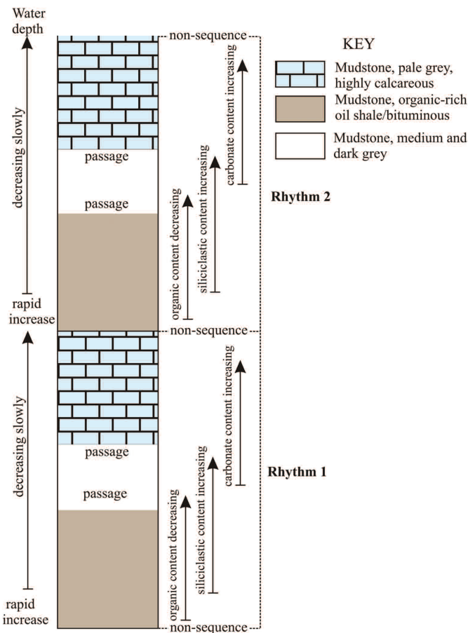
Figure 4. Generalised small-scale (fourth order) Kimmeridge Clay Type B (organic-rich) rhythm (after Cox and Gallois, 1981).
