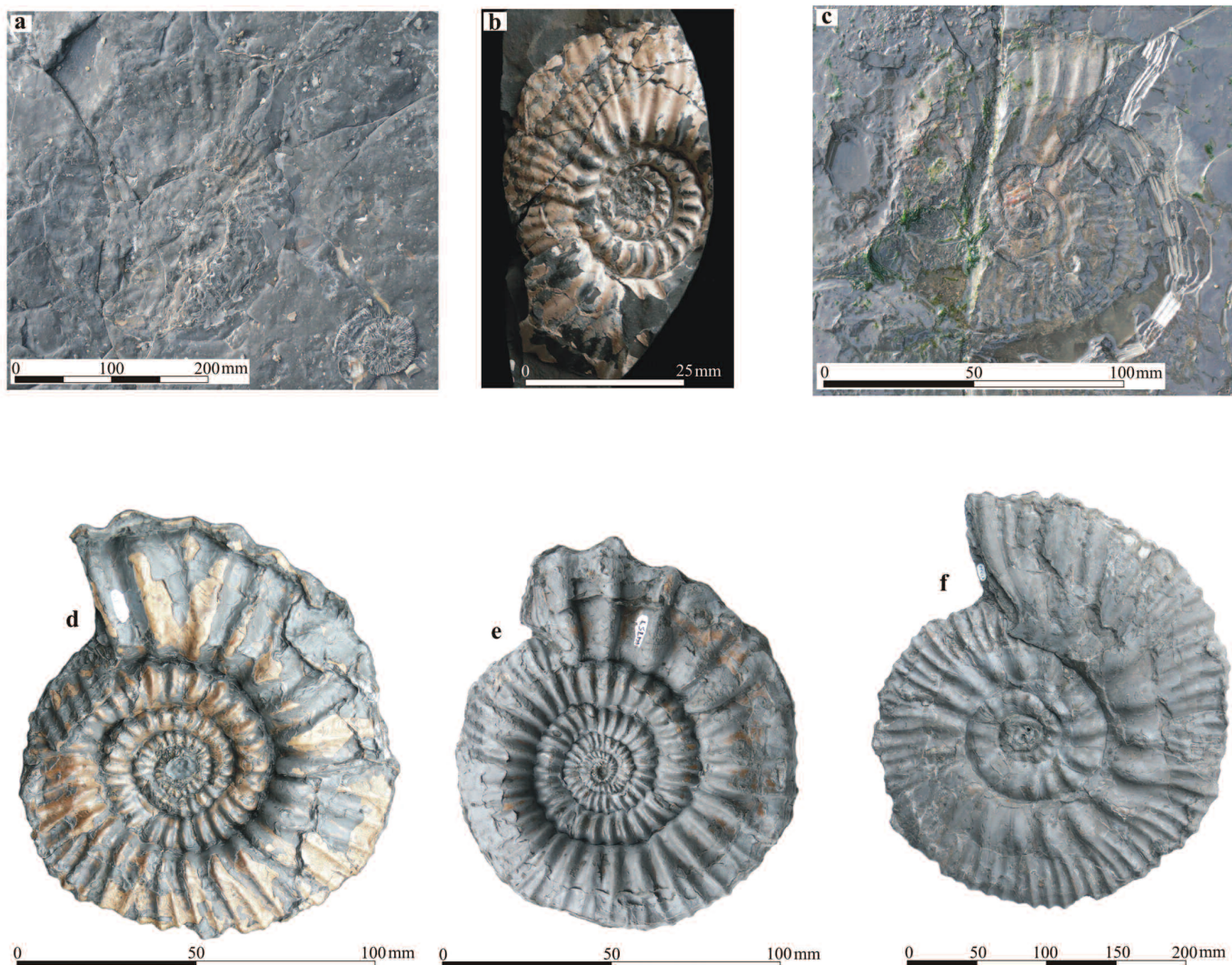
Figure 7. Examples of Gravesia preservation, and well-preserved examples from the autissiodorensis Zone in the Kimmeridge area. (a) Solution worn and eroded macroconch cf. G. gigas or G. gravesiana , Bed M 14, foreshore below Hen Cliff. (b) Inner whorls “close to G. polypleura ” (Hantzpergue and Lafaurie, 1986), Kimmeridge Bay Borehole at 23.30 m depth; BGS- GSM 118161, Bed W 20, autissiodorensis Zone. (c) Crushed and fractured G. cf. gravesiana , Bed Y2, scitulus Zone, foreshore below Cuddle. (d) Possible microconch of an early, undescribed form of Gravesia ; K1581, Bed W13, autissiodorensis Zone, foreshore in Brandy Bay; more evolute than macrochonchiate forms of Gravesia . (e) Microconch of possible early form of Gravesia with well developed lappet, K1757, Bed W20, foreshore in Kimmeridge Bay, autissiodorensis Zone at a similar stratigraphical level to (b) . (f) G. cf. gravesiana (M), K1078, Bed M10, autissiodorensis Zone, foreshore in Brandy Bay.
