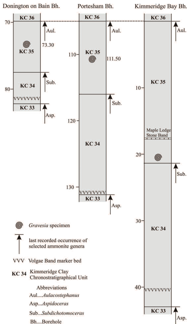
Figure 10. Comparison of the stratigraphical positions of the Gravesia recorded in the Donington on Bain (Lincolnshire), Portesham (Dorset) and Kimmeridge Bay (Dorset) boreholes.
