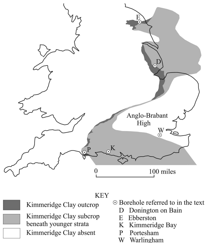
Figure 1. Geological sketch map of the English outcrop and subcrop of the Kimmeridge Clay Formation.
