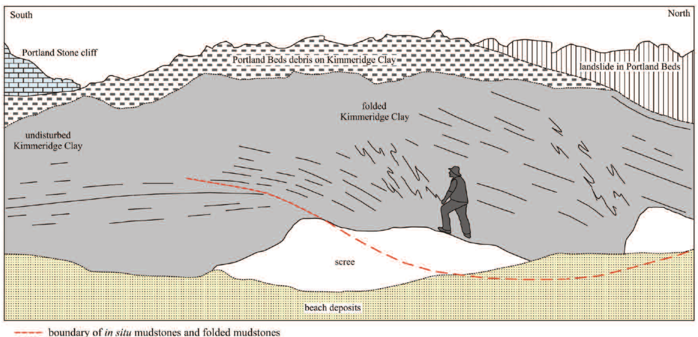
Figure 5. Contact of undisturbed and periglacially folded Kimmeridge Clay Formation mudstones: outcrop below Grove Coastguard Station, Isle of Portland.
