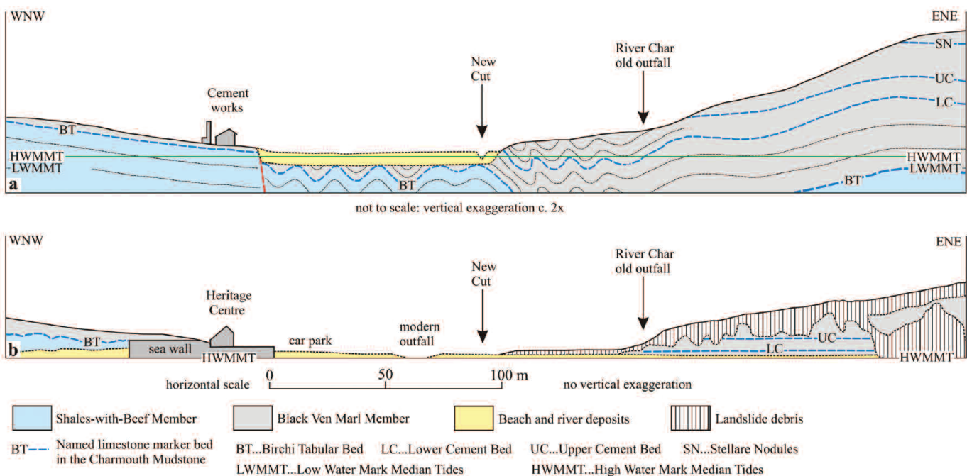
Figure 2. Geological sketch sections to illustrate folding and faulting in the Charmouth Mudstone adjacent to the outfall of the River Char at Charmouth. (a) The "Char Valley Disturbance": redrawn from Lang 1914, fig. 23A. (b) Section based on photographs taken normal to the cliff line at low spring tide in September 2010.
