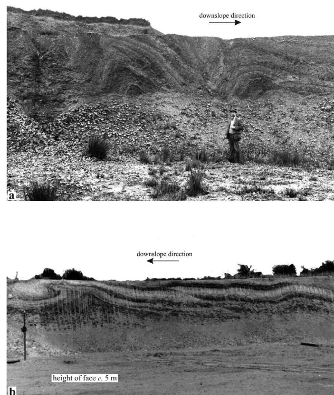
Figure 10. Folds in Cretaceous Weald Clay Formation at the former Southwater Brickpit, Horsham Sussex. (a) View south west, May 1931, BGS A05368. (b) View east, July 1949, A 08320. Photographs by the late J. Rhodes. Reproduced with the permission of the British Geological Survey ©NERC. All rights Reserved.
