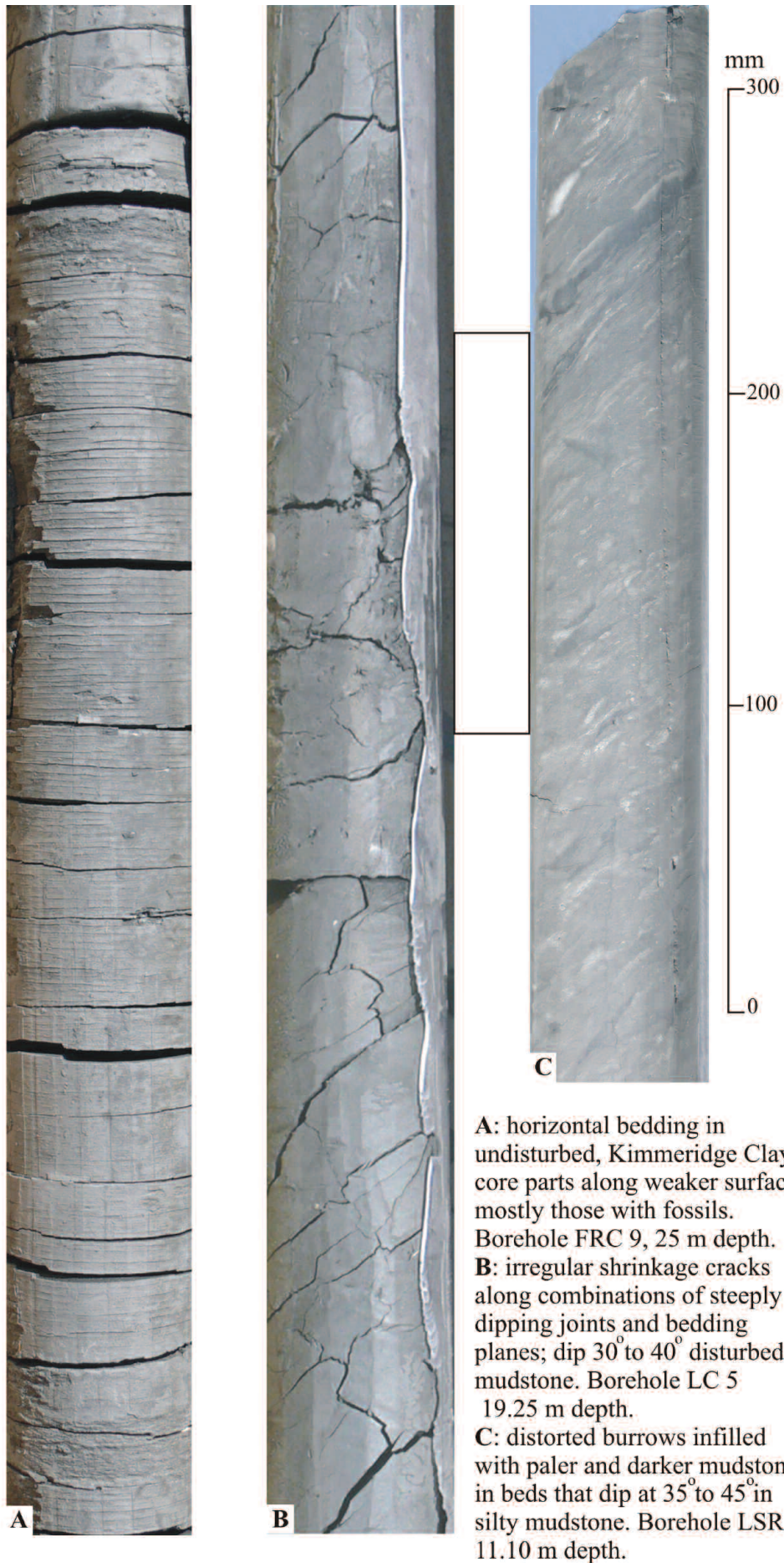
Figure 4. Examples of undisturbed (a) and disturbed (b and c) bedding in borehole cores in Kimmeridge Clay, Upper Osprey site, Isle of Portland.
