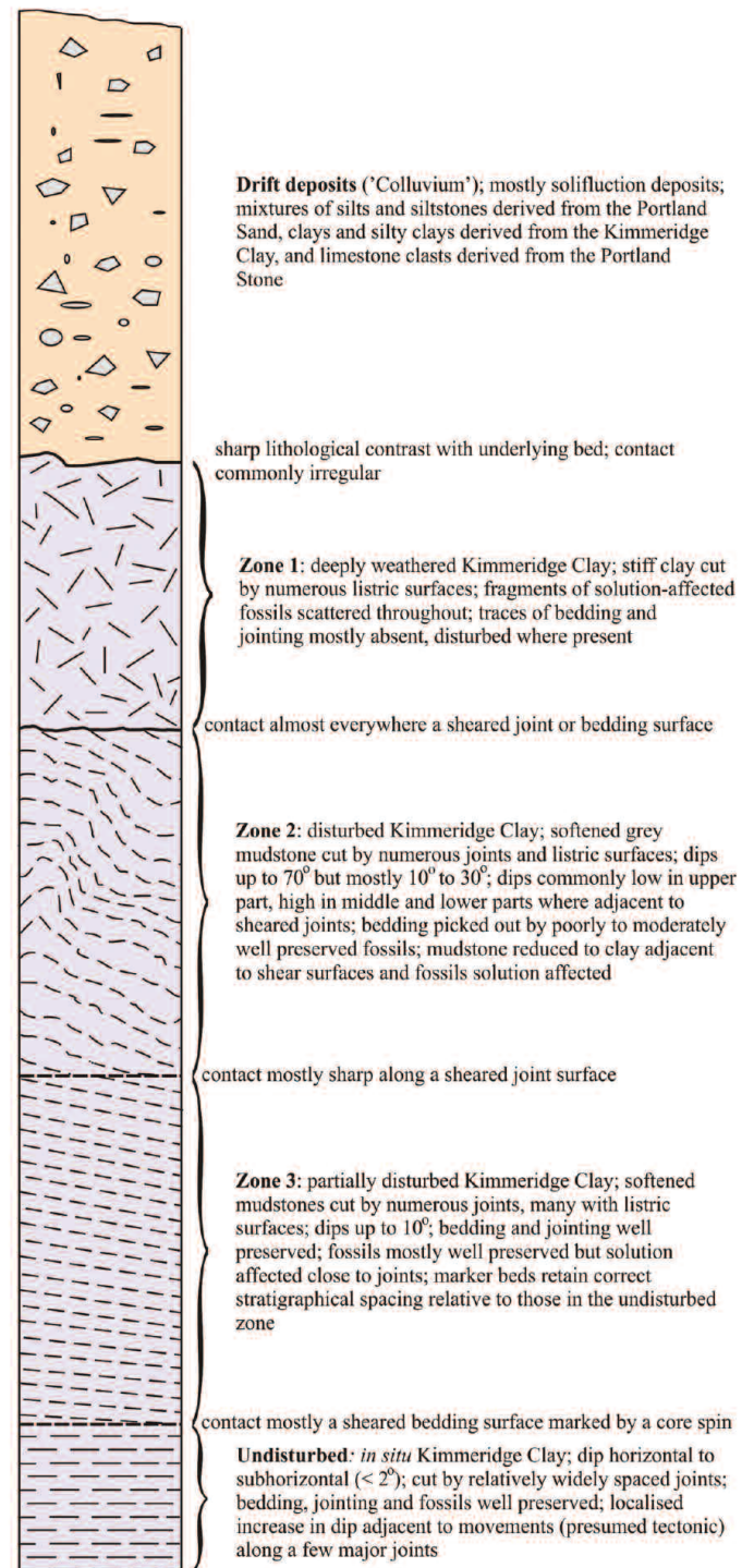
Figure 3. Generalised weathering and deformation profile for the near-surface layers of the Kimmeridge Clay at the Upper Osprey site on the Isle of Portland.
