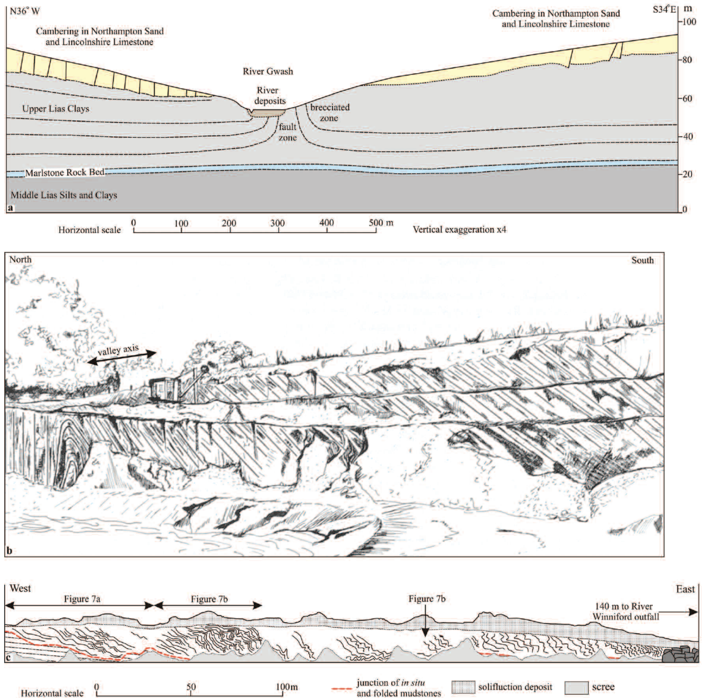
Figure 9. Geological sketch sections to illustrate the differences in gross morphology between valley bulges and large-scale periglacial folding. (a) Valley bulge in Upper Lias Clays (now Charmouth Mudstone) and associated cambering in the Northampton Sand and Lincolnshire Limestone formations in the Gwash Valley, Lincolnshire (after Horswill et al. , 1976). (b) Detail of the central part of a valley bulge in the Cretaceous Wadburst Clay Formation showing the characteristic intense deformation along the valley axis and a steady decline in dip angle away from the axis. Freshfield Lane Brickworks, Danehill, Sussex based on BGS Photograph A 10249 oblique to the quarry face: excavator arm c. 7 m high (after Gallois and Worssam, 1993, fig.29). (c) Progressive downslope deformation in the periglacially folded Green Ammonite Member mudstones at Seatoun based on photographs taken in 2007 to 2010: uncorrected for parallax and perspective.
