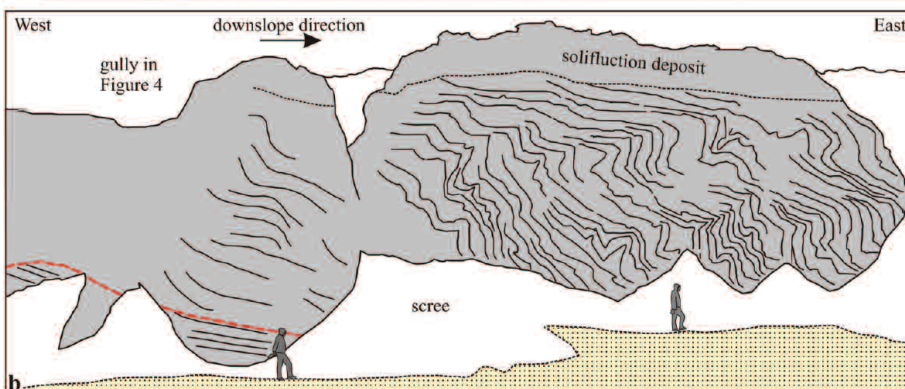
Figure 8. (a) The junction of in situ eastward dipping Green Ammonite Member mudstones and the periglacially folded mudstones, 300 m west of outfall of River Winniford, Seatown. Photographed on December 30th 1007 when the sections were particularly well exposed: uncorrected for parallax and perspective. Figure 1.8 m high: maximum cliff height 18 m. (b) Intensely folded and partially overturned Green Ammonite Member mudstones 50 m east of (a): uncorrected for parallax and perspective. Figure 1.8 m high: maximum cliff height 20 m. (c) Detail of kink bands in mudstones 200 m east of (a): axe 0.7 m long.
